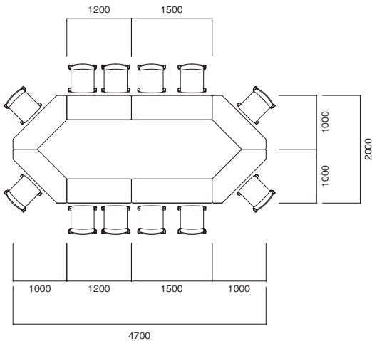
■ Layout Plan-1
